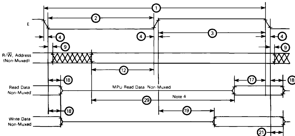
FIGURE 2 — BUS TIMING
