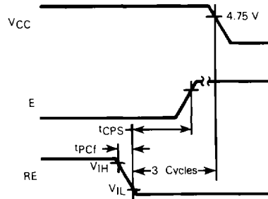
FIGURE 10 — POWER-DOWN SEQUENCE
