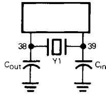
FIGURE 12 — CRYSTAL SPECIFICATIONS
