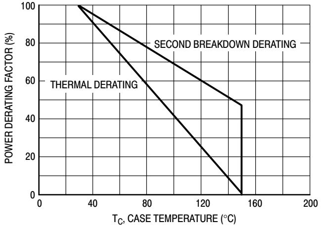
Figure 21. Power Derating
