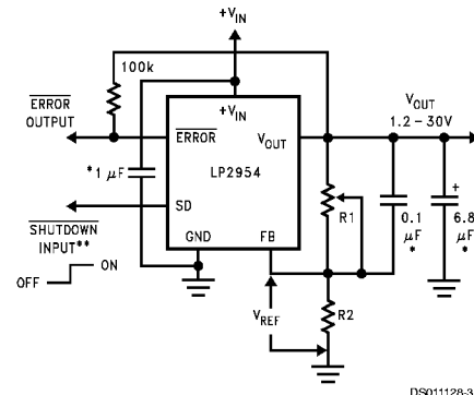
FIGURE 2. Adjustable Regulator
