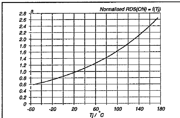
Fig. 9. Normalised drain-source on-state resistance. a = R_{DS(ON)}/R_{DS(ON)25 \text{ }^\circ\text{C}} = f(T_j) ; I_D = 7 \text{ A} ; V_{GS} = 10 \text{ V}
