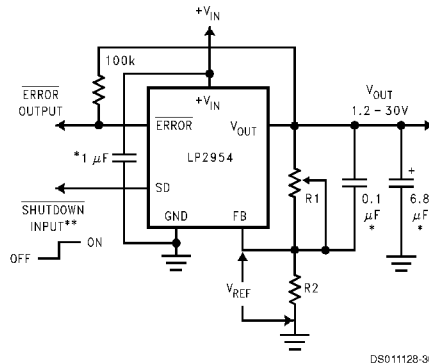
FIGURE 2. Adjustable Regulator
