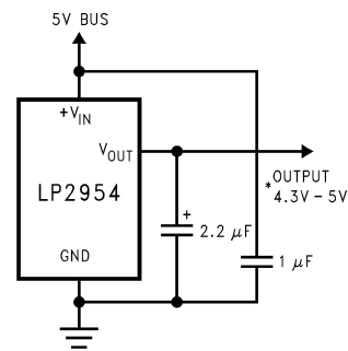
Figure 27. 5V Regulator
