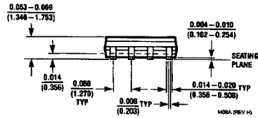
8-Lead (0.150" Wide) Molded Small Outline Package, JEDEC Order Number LM6132AIM, LM6132BIM, LM6132AIMX or LM6132BIMX NS Package Number M08A
