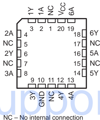
SN54HC14 . . . FK PACKAGE (TOP VIEW)
