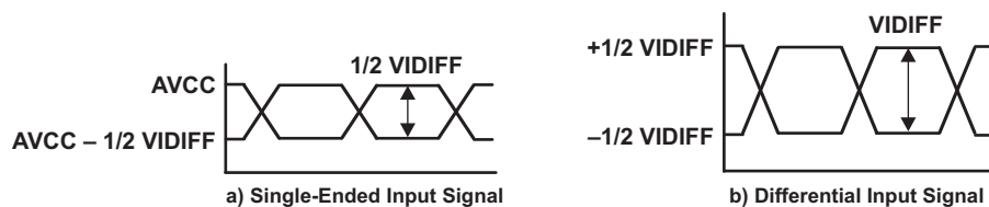
Figure 16. TMD5 Inputs
