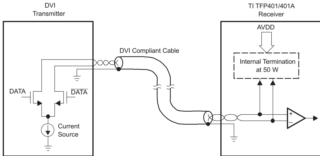
Figure 15. TMD5 Differential Input and Transmitter Connection
