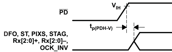
Figure 8. Delay From \overline{\text{PD}} Low to High Until Inputs Are Active
