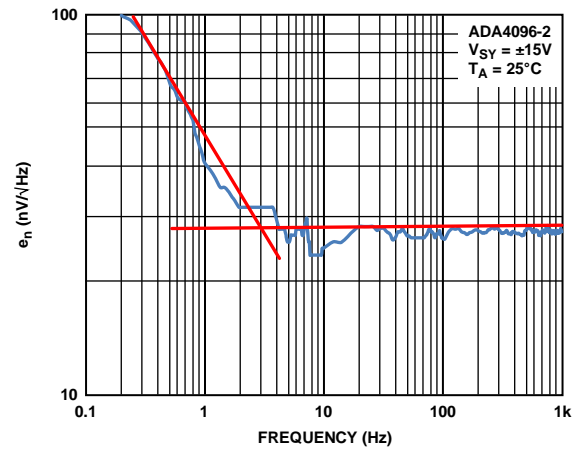
Figure 43. Voltage Noise Density
