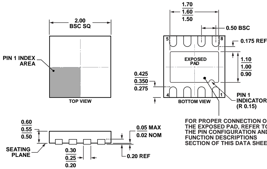
Figure 50. 8-Lead Lead Frame Chip Scale Package [LFCSP_UD]
