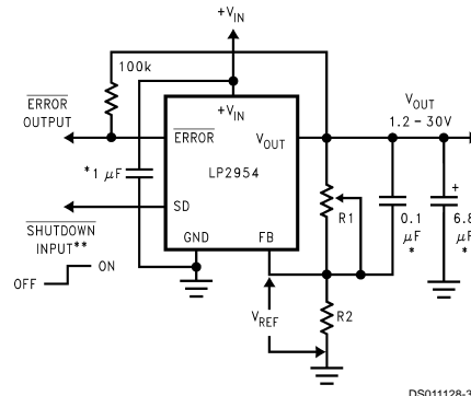
FIGURE 2. Adjustable Regulator
