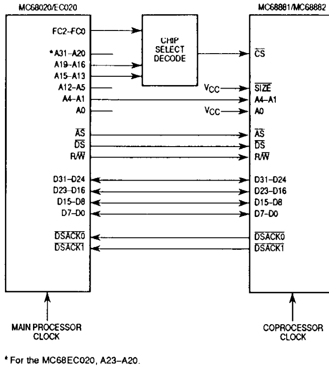
Figure 9-1. 32-Bit Data Bus Coprocessor Connection
