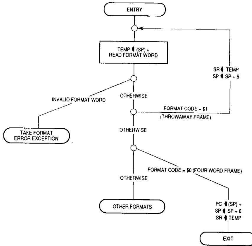
Figure 6-7. RTE Instruction for Throwing Four-Word Frame
