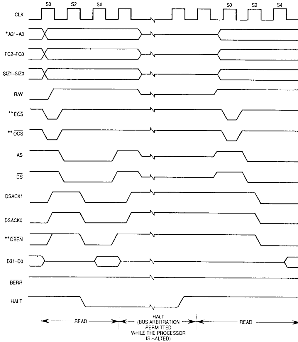
Figure 5-41. Halt Operation Timing
