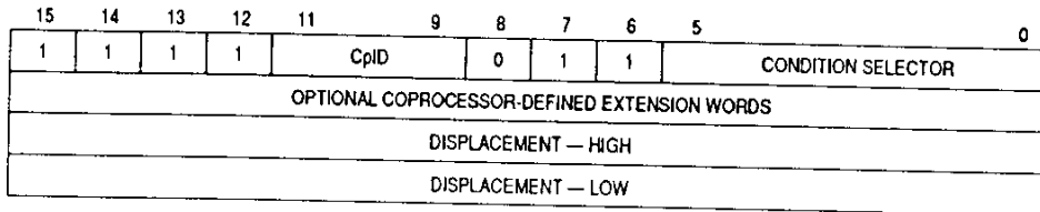
Figure 7-10. Branch on Coprocessor Condition Instruction Format (cpBcc.L)
