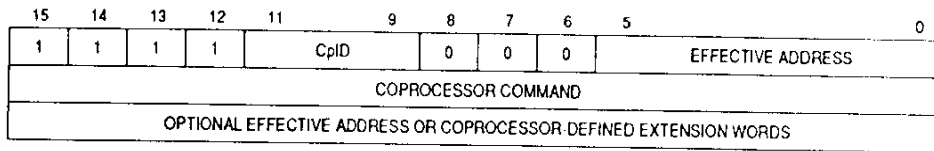
Figure 7-6. Coprocessor General Instruction Format (cpGEN)
