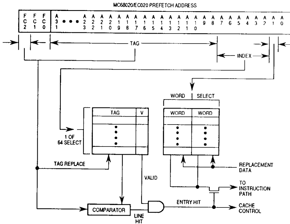
Figure 4-1. MC68020/EC020 On-Chip Cache Organization
