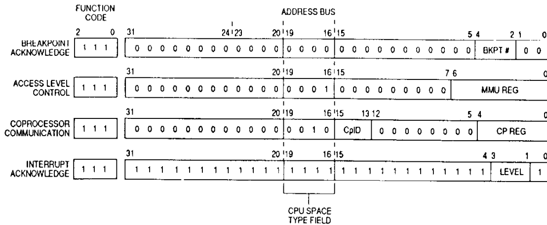
Figure 5-31. MC68020/EC020 CPU Space Address Encoding
