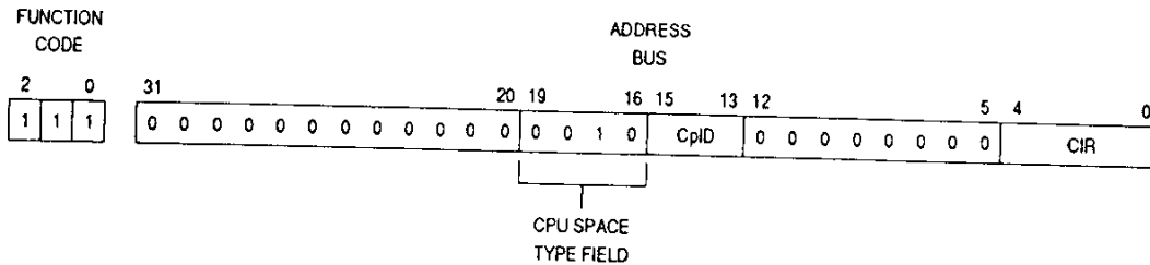
Figure 7-3. MC68020/EC020 CPU Space Address Encodings
