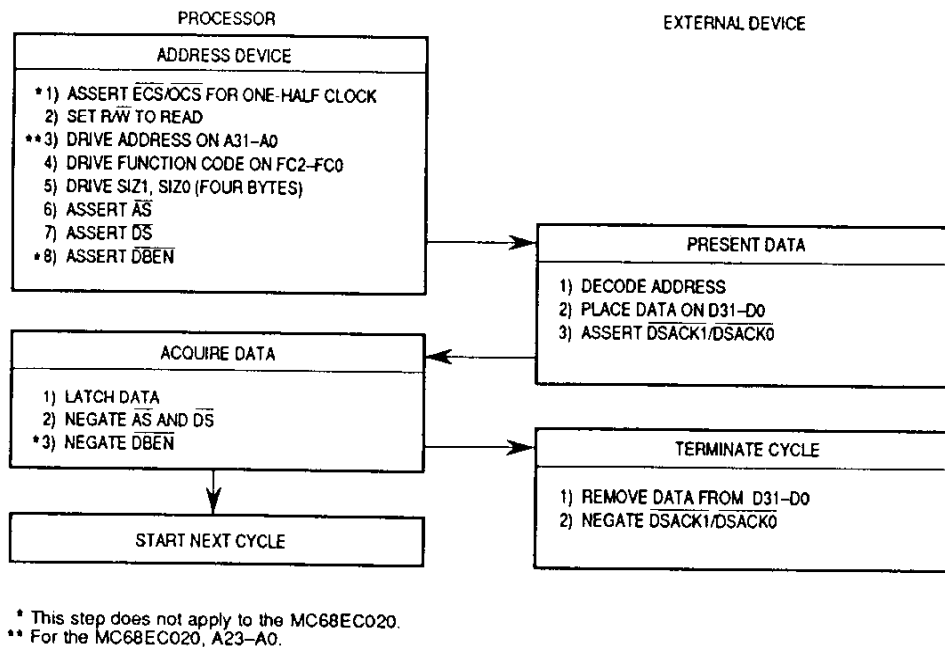
Figure 5-19. Long-Word Read Cycle Flowchart
