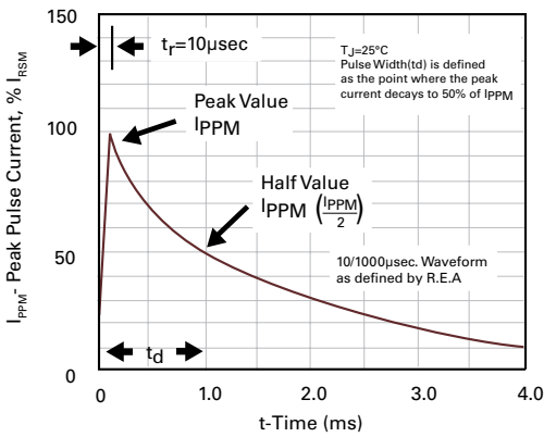
Figure 3 - Pulse Waveform
