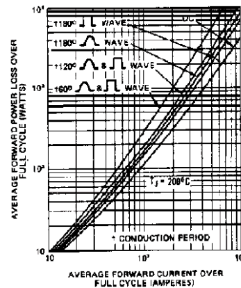
Fig. 8 - Maximum High Level Forward Power Loss vs. Average Forward Current, 1N1183A Series
