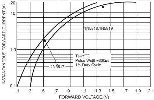
FIG.3-TYPICAL FORWARD CHARACTERISTICS
