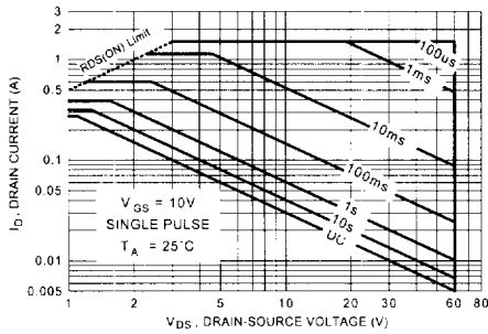
Figure 15. NDS7000A Maximum Safe Operating Area.
