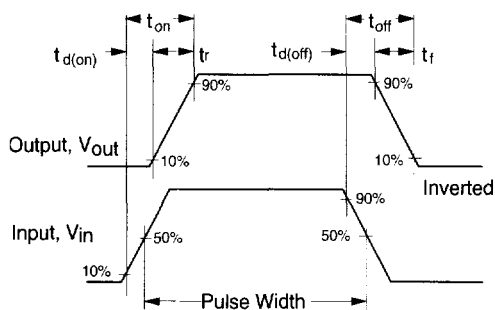
Figure 12. Switching Waveforms.
